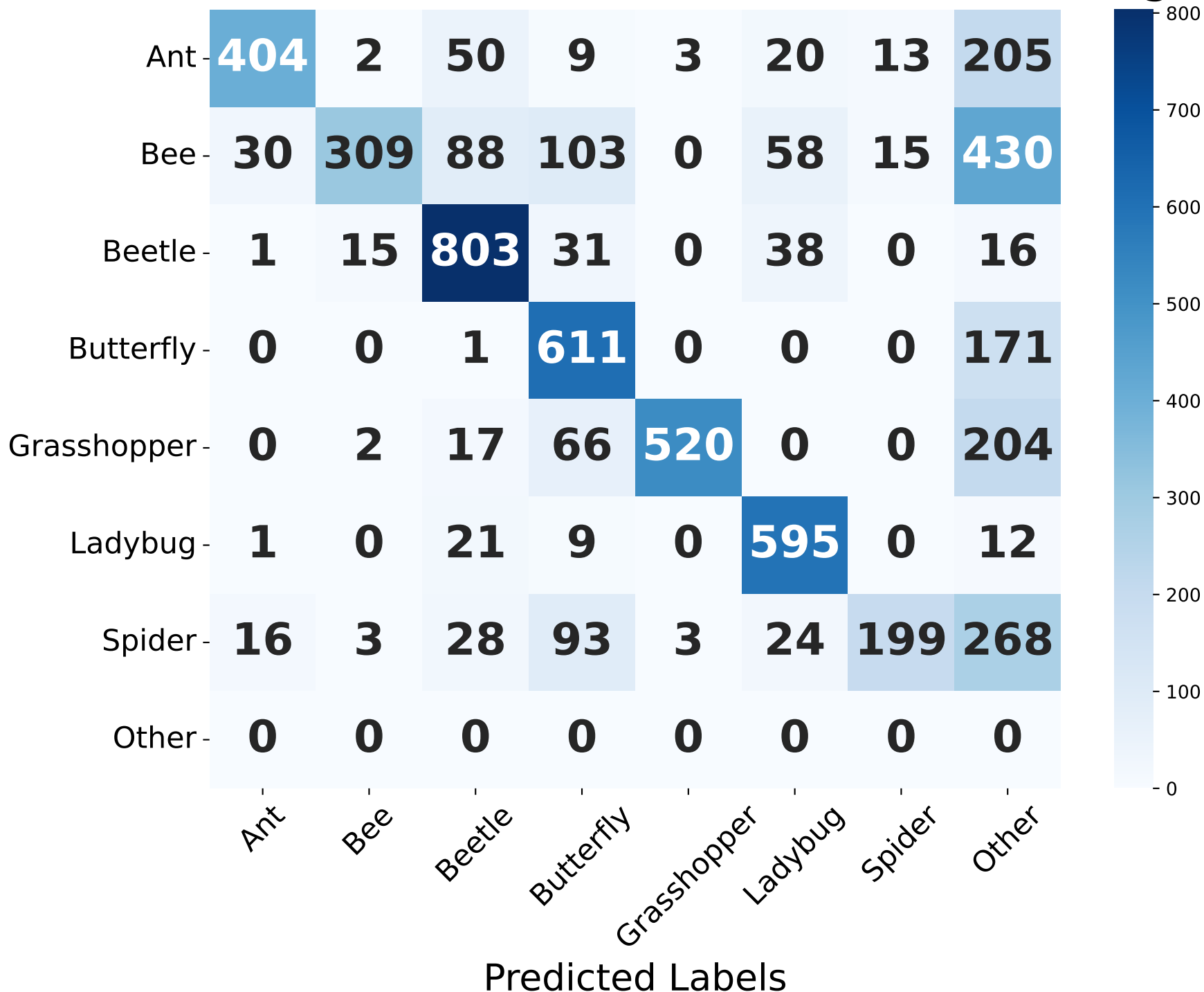
Confusion Matrix: Full iNat (Partial Unfreezing)
